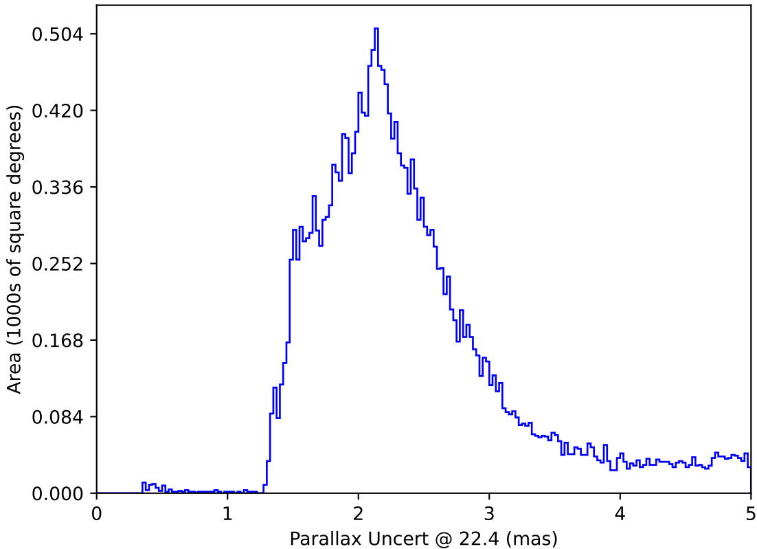
noroll_mjdp60_v3.4_10yrs All sky: Parallax Uncert @ 22.4
