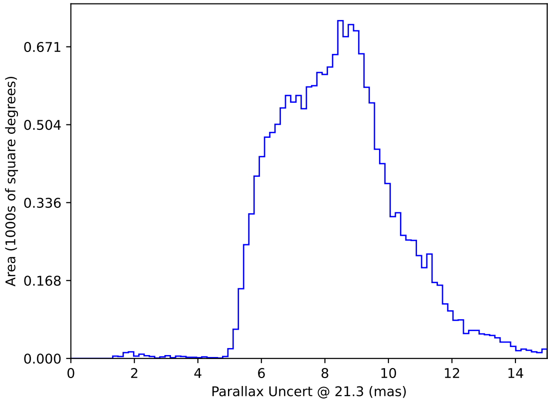
noroll_mjdp60_v3.4_10yrs WFD y band only: Parallax Uncert @ 21.3
