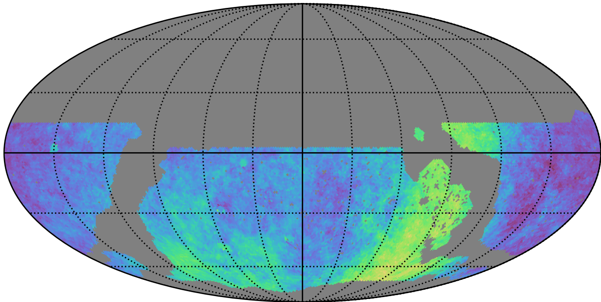
noroll_mjdp60_v3.4_10yrs WFD: Parallax Coverage @ 24.0
