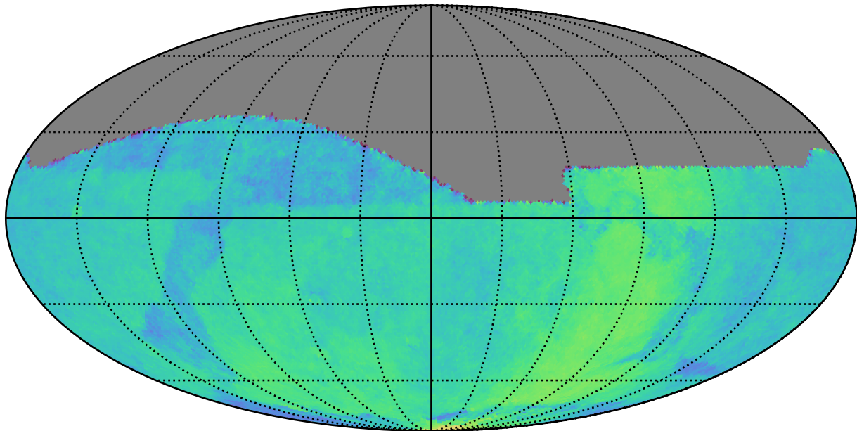
noroll_mjdp60_v3.4_10yrs All sky: Parallax Coverage @ 24.0
