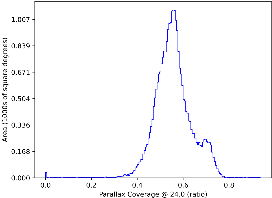
noroll_mjdp60_v3.4_10yrs All sky: Parallax Coverage @ 24.0
