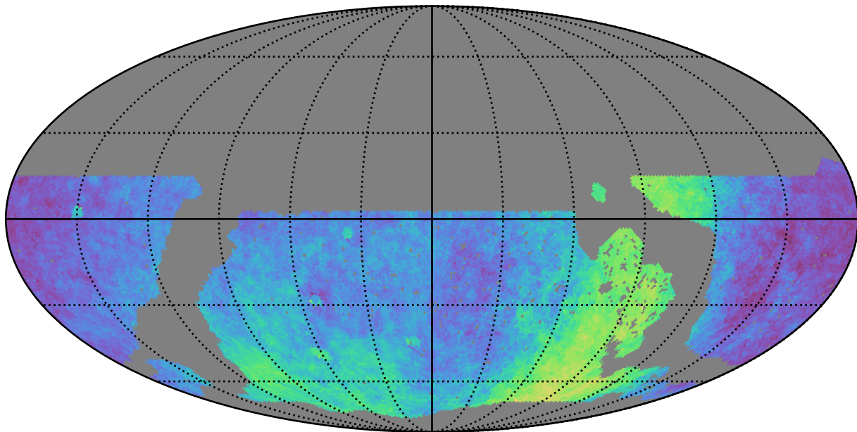
noroll_mjdp60_v3.4_10yrs WFD: Parallax Coverage @ 22.4
