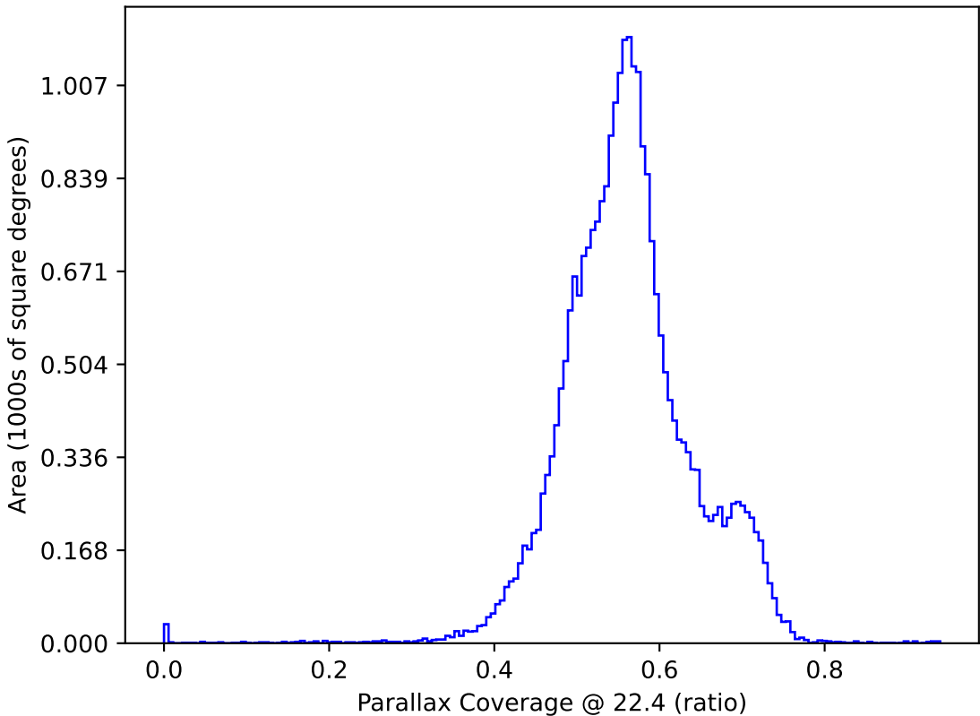
noroll_mjdp60_v3.4_10yrs All sky: Parallax Coverage @ 22.4
