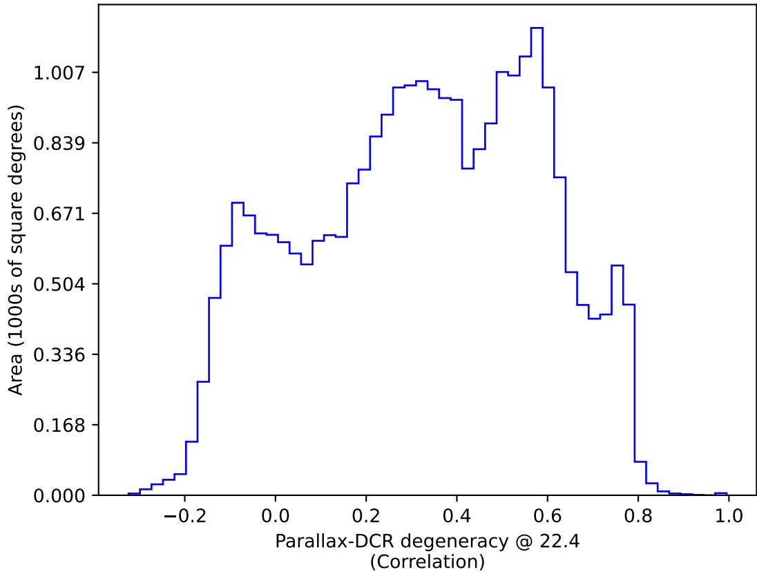
noroll_mjdp60_v3.4_10yrs All sky: Parallax-DCR degeneracy @ 22.4
