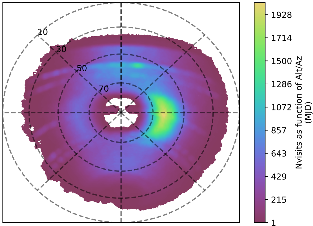
noroll_mjdp60_v3.4_10yrs y band: Nvisits as function of Alt/Az
