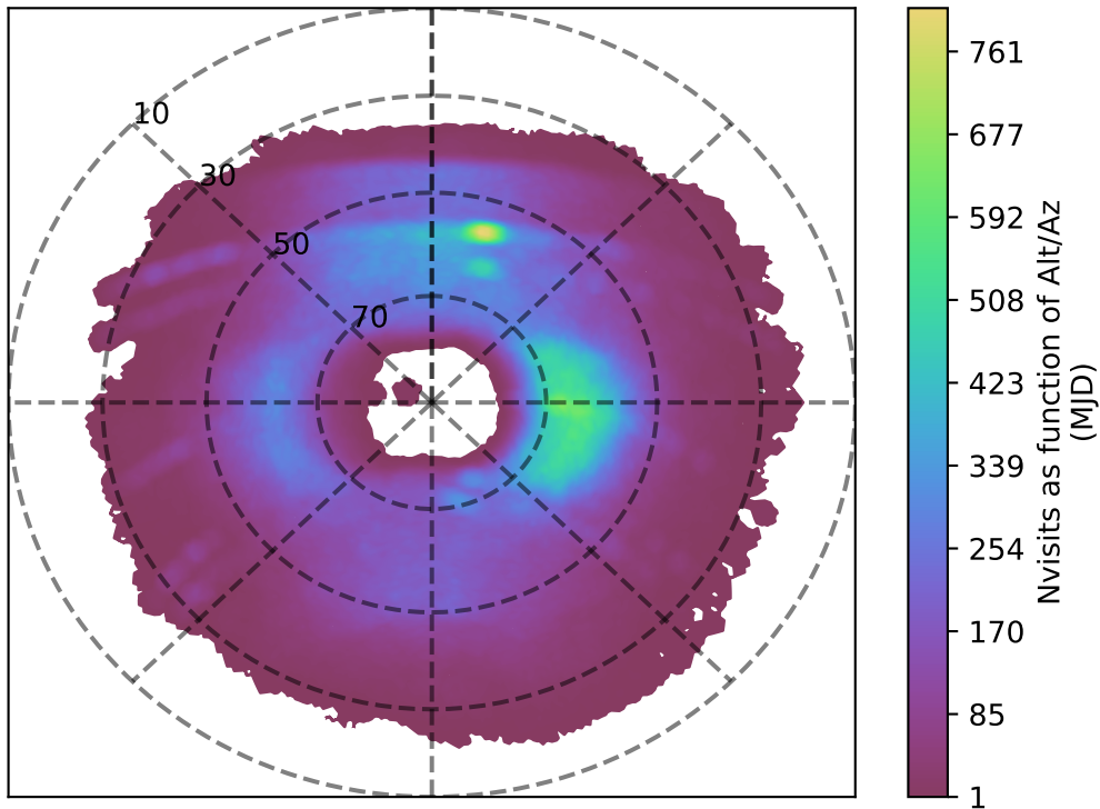
noroll_mjdp60_v3.4_10yrs u band: Nvisits as function of Alt/Az
