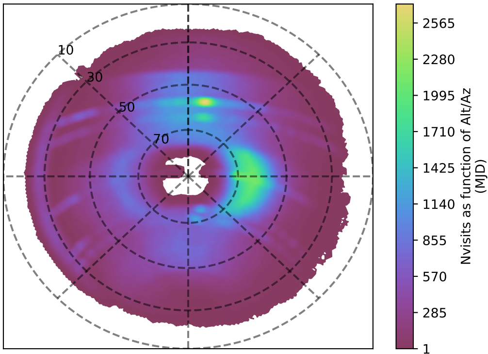
noroll_mjdp60_v3.4_10yrs r band: Nvisits as function of Alt/Az
