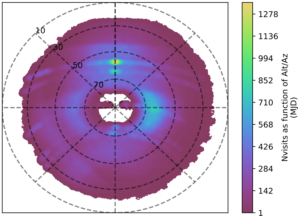
noroll_mjdp60_v3.4_10yrs g band: Nvisits as function of Alt/Az
