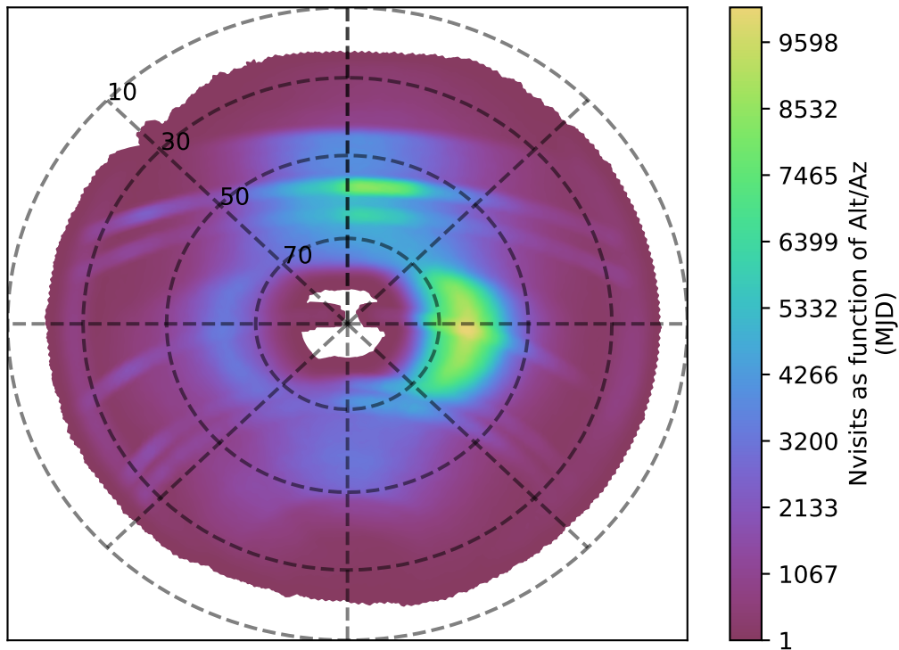
noroll_mjdp60_v3.4_10yrs all bands: Nvisits as function of Alt/Az
