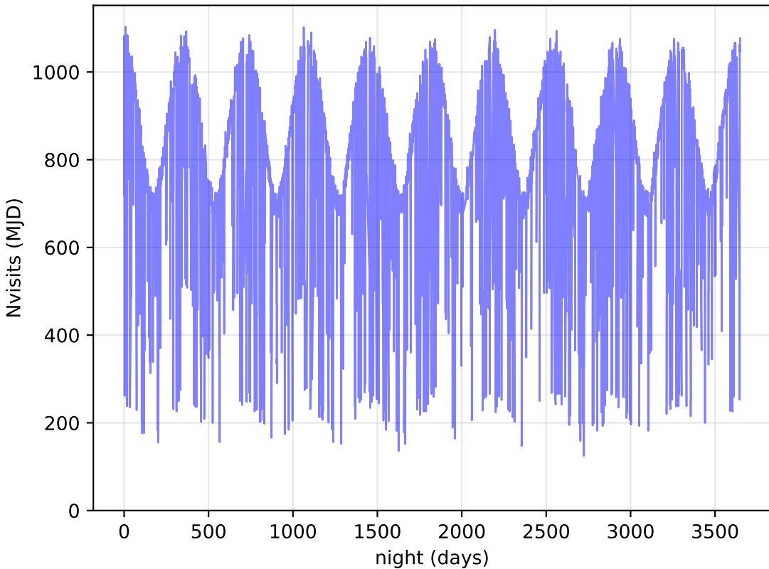
noroll_mjdp60_v3.4_10yrs All visits: Nvisits
