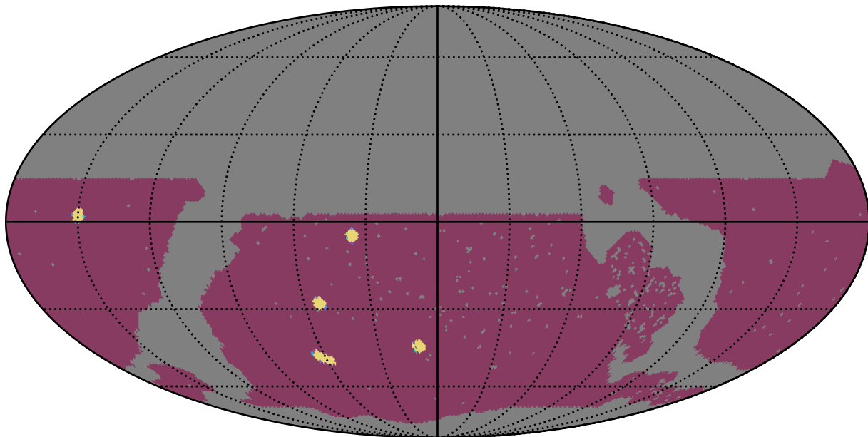
noroll_mjdp60_v3.4_10yrs WFD: NumberOfQuickRevisits
