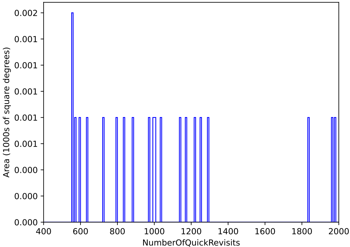
noroll_mjdp60_v3.4_10yrs WFD: NumberOfQuickRevisits
