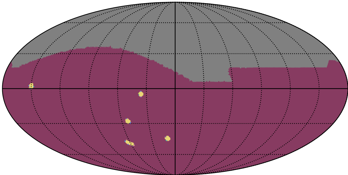
noroll_mjdp60_v3.4_10yrs All sky: NumberOfQuickRevisits
