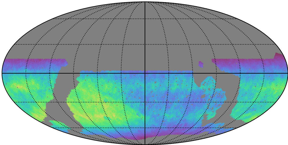
noroll_mjdp60_v3.4_10yrs WFD z band: Normalized Teff
