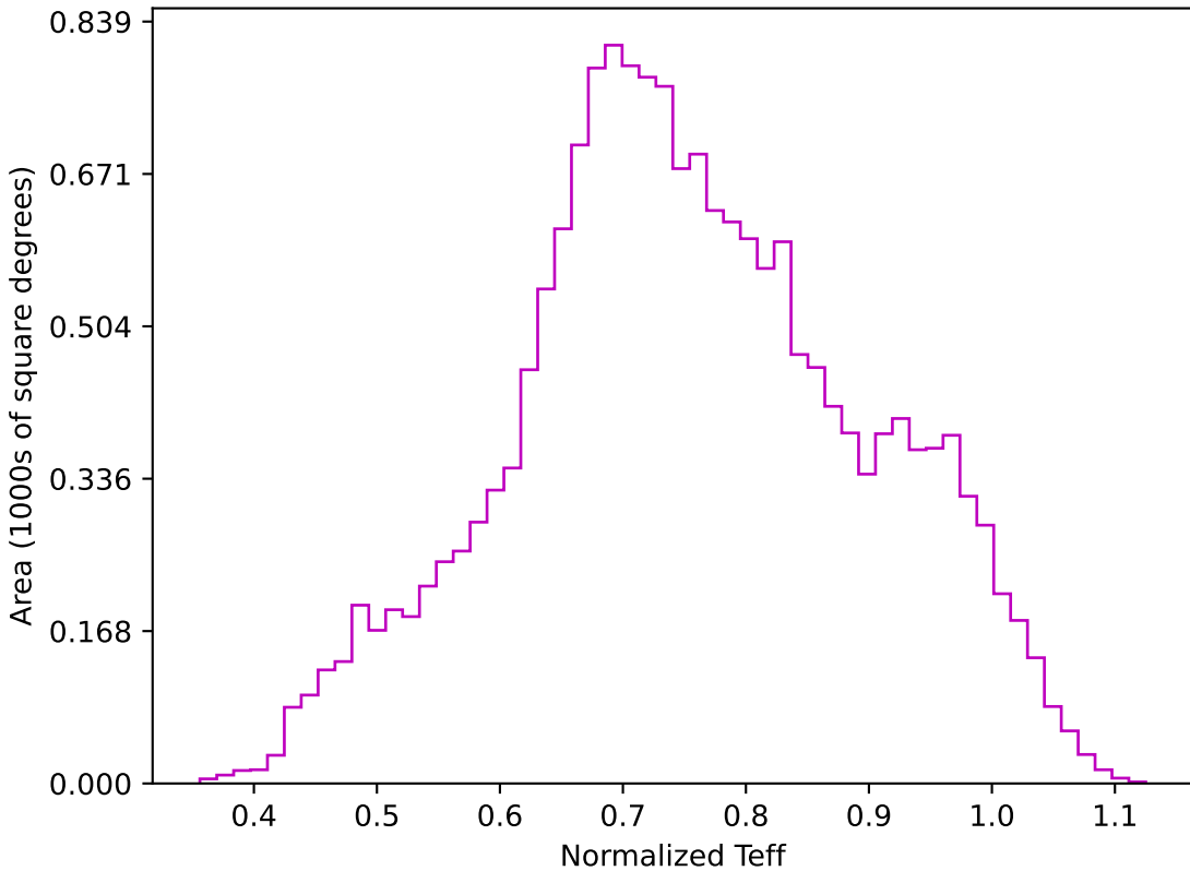
noroll_mjdp60_v3.4_10yrs WFD z band: Normalized Teff
