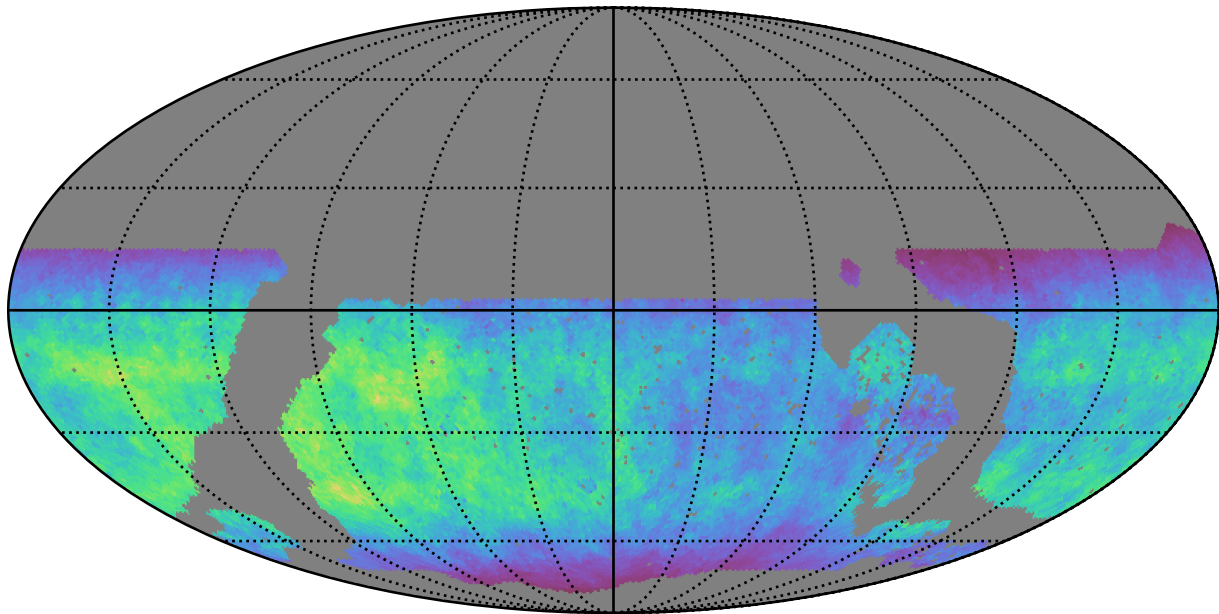
noroll_mjdp60_v3.4_10yrs WFD u band: Normalized Teff
