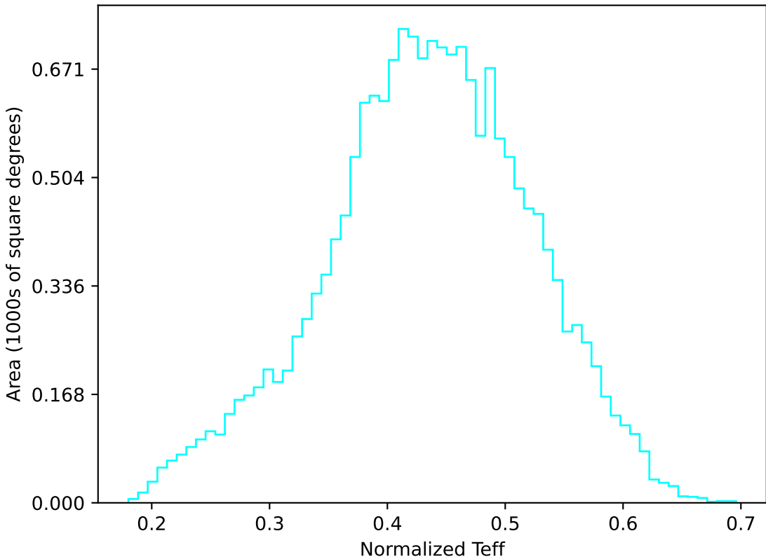
noroll_mjdp60_v3.4_10yrs WFD u band: Normalized Teff
