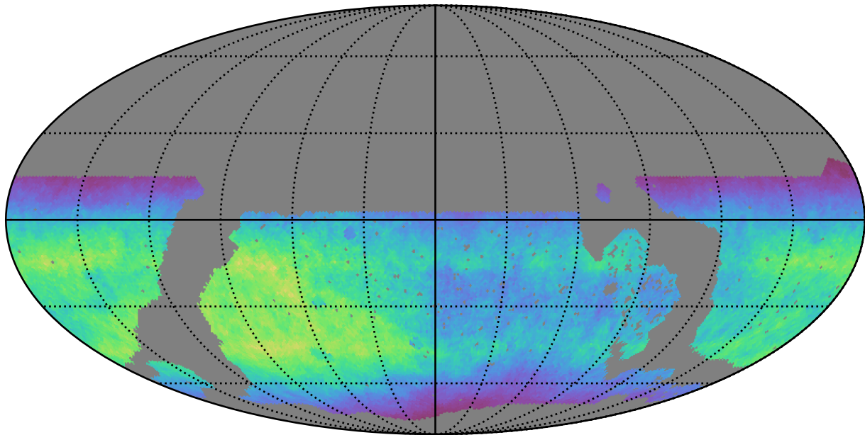
noroll_mjdp60_v3.4_10yrs WFD i band: Normalized Teff
