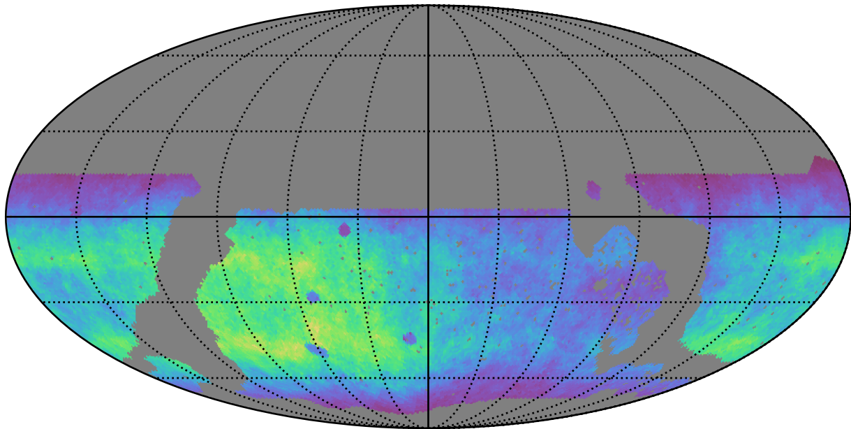
noroll_mjdp60_v3.4_10yrs WFD g band: Normalized Teff
