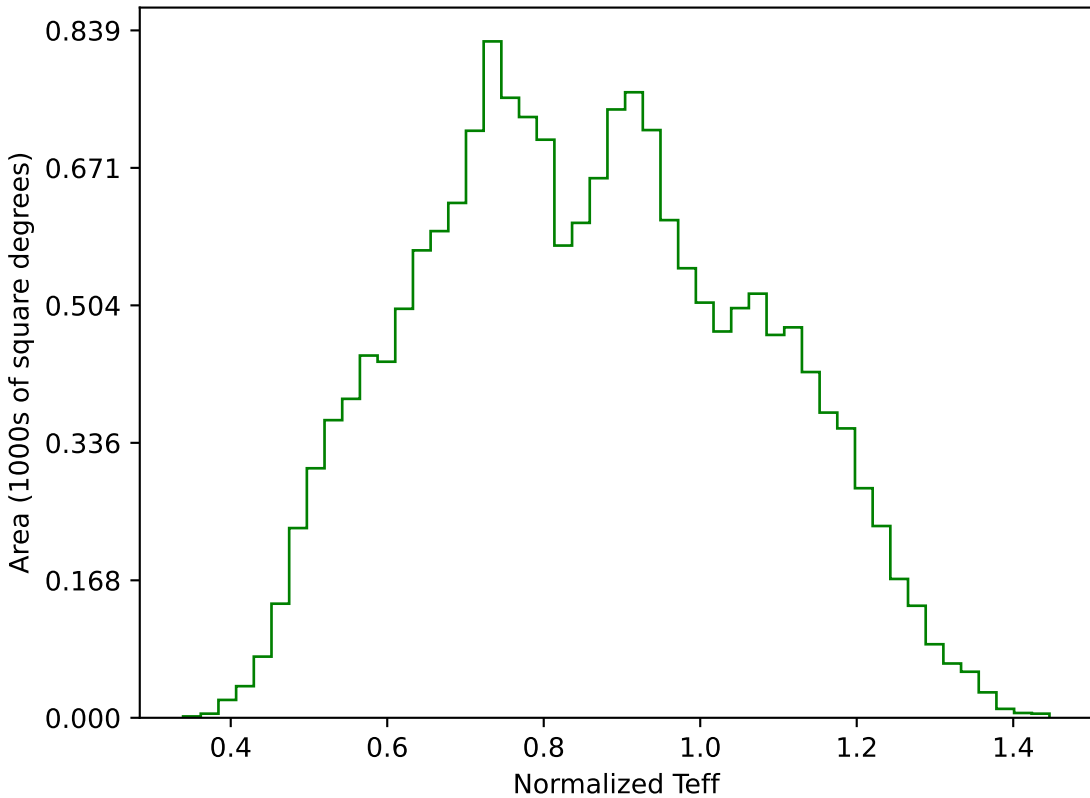
noroll_mjdp60_v3.4_10yrs WFD g band: Normalized Teff
