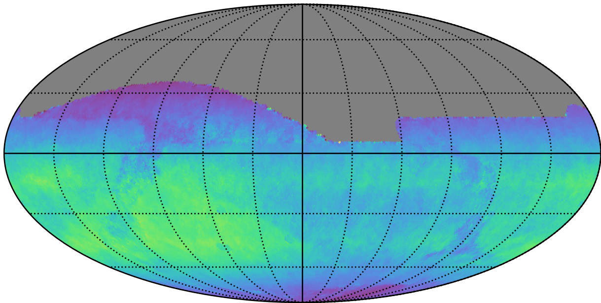
noroll_mjdp60_v3.4_10yrs All sky z band: Normalized Teff
