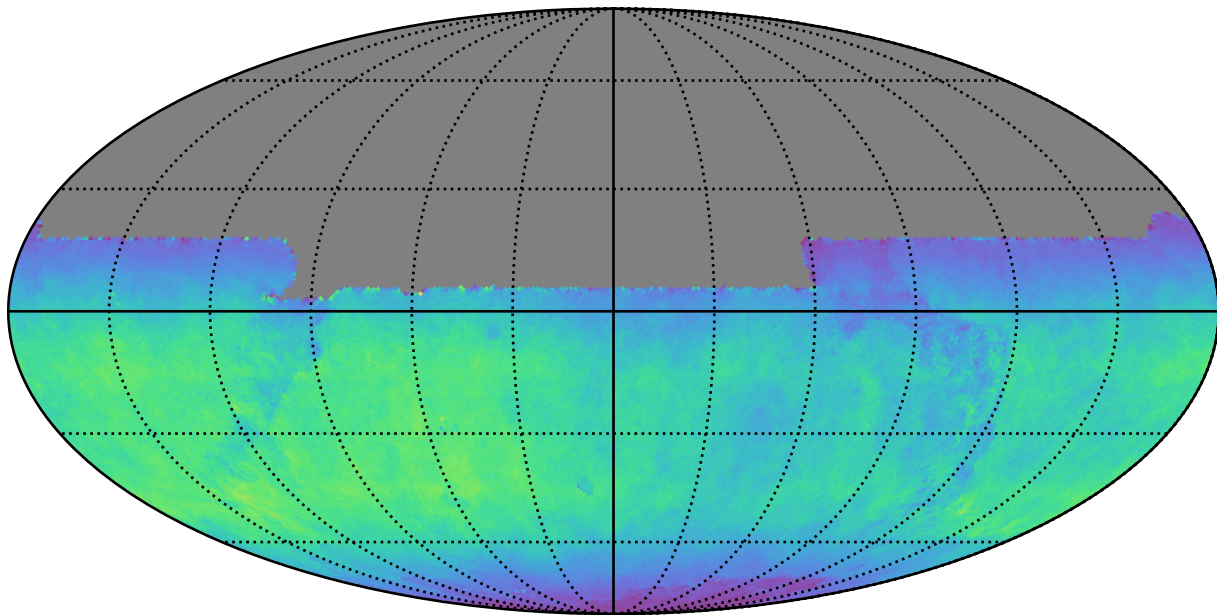
noroll_mjdp60_v3.4_10yrs All sky y band: Normalized Teff
