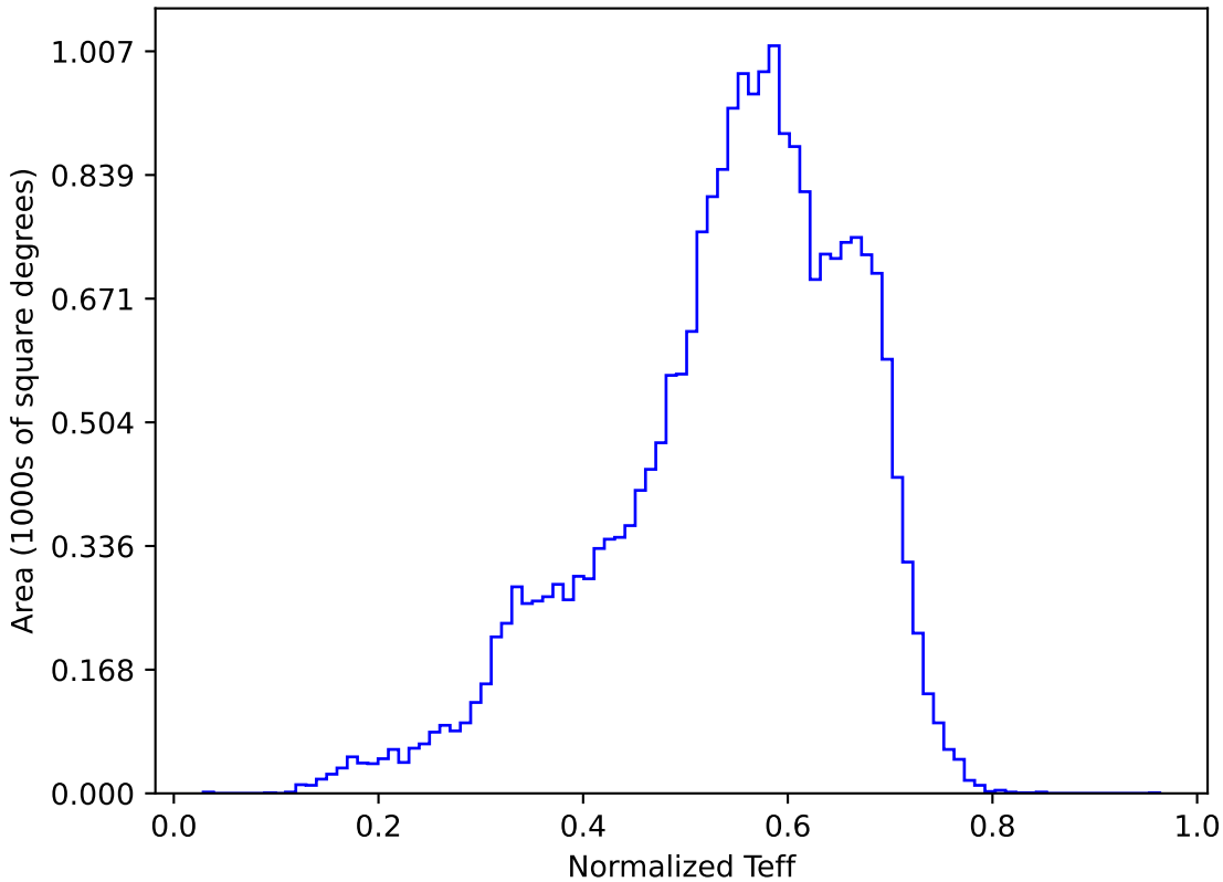
noroll_mjdp60_v3.4_10yrs All sky y band: Normalized Teff
