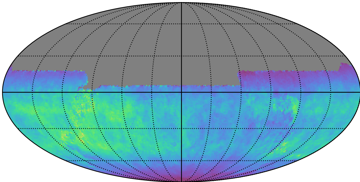
noroll_mjdp60_v3.4_10yrs All sky u band: Normalized Teff
