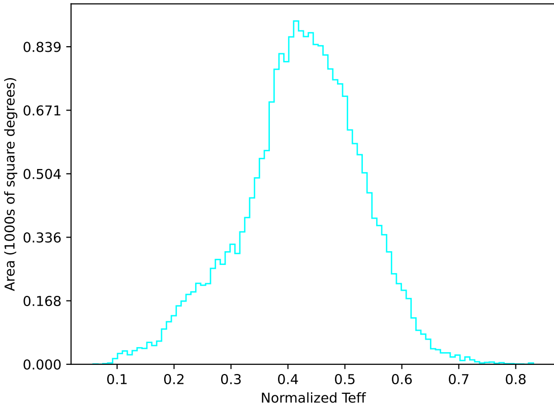
noroll_mjdp60_v3.4_10yrs All sky u band: Normalized Teff
