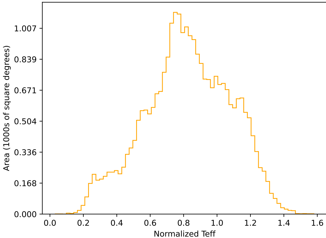
noroll_mjdp60_v3.4_10yrs All sky r band: Normalized Teff
