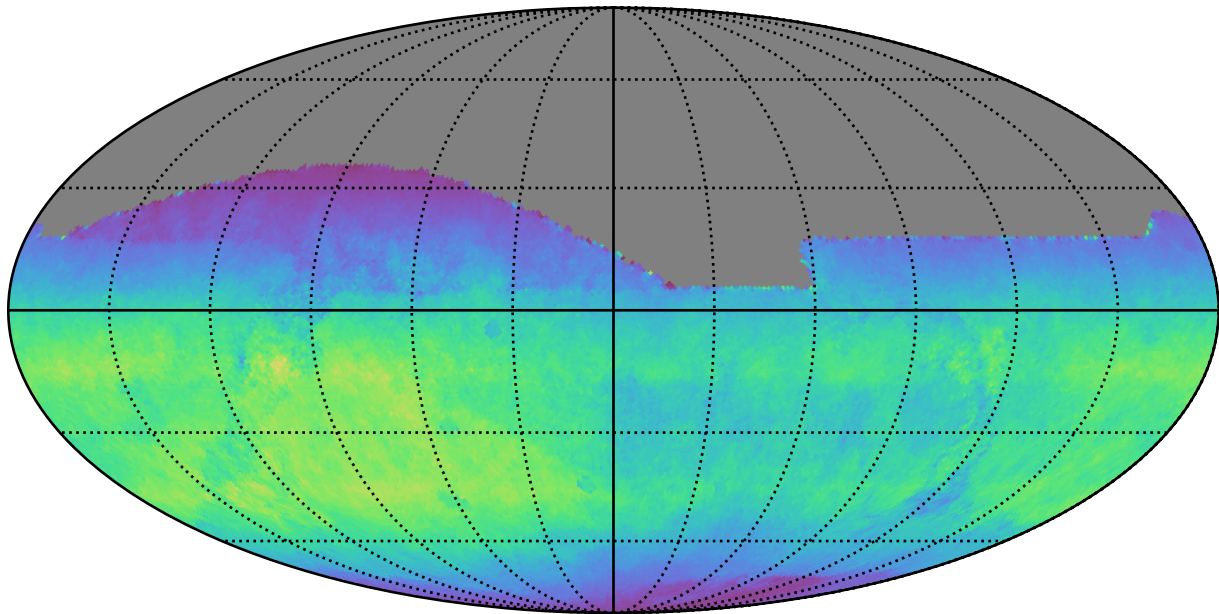
noroll_mjdp60_v3.4_10yrs All sky i band: Normalized Teff
