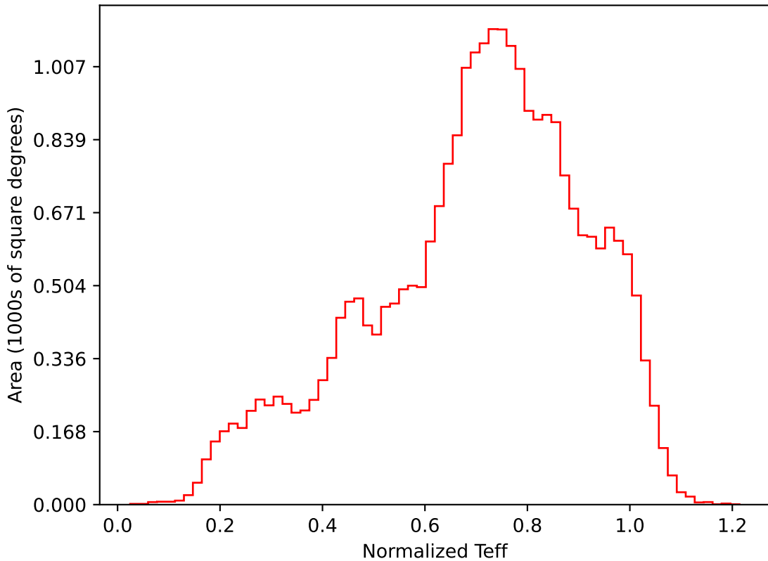
noroll_mjdp60_v3.4_10yrs All sky i band: Normalized Teff
