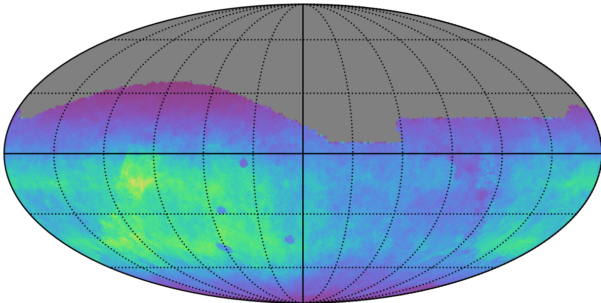
noroll_mjdp60_v3.4_10yrs All sky g band: Normalized Teff
