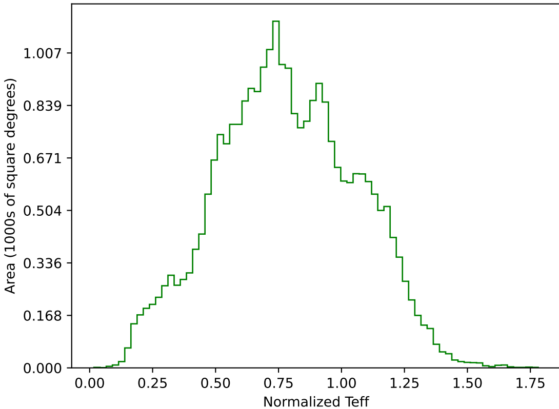
noroll_mjdp60_v3.4_10yrs All sky g band: Normalized Teff
