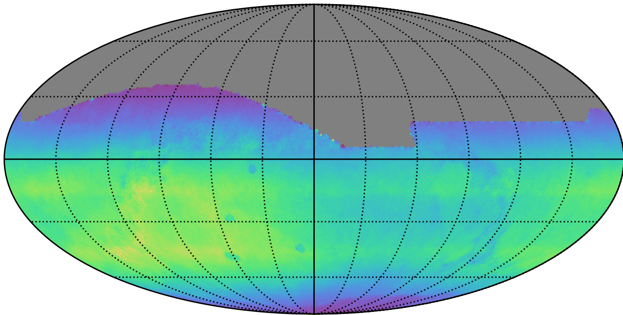
noroll_mjdp60_v3.4_10yrs All sky all bands: Normalized Teff
