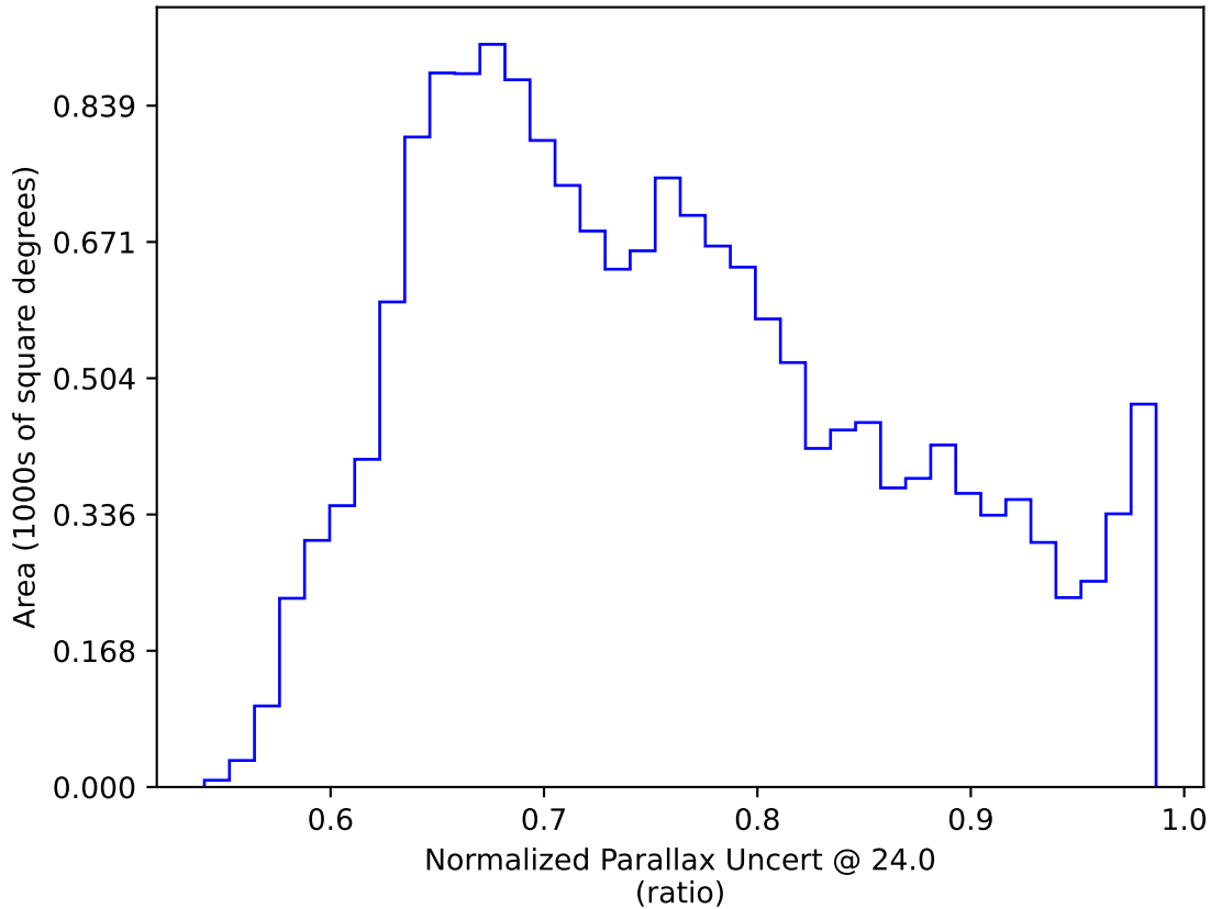
noroll_mjdp60_v3.4_10yrs WFD: Normalized Parallax Uncert @ 24.0
