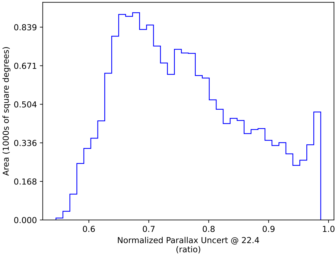
noroll_mjdp60_v3.4_10yrs WFD: Normalized Parallax Uncert @ 22.4
