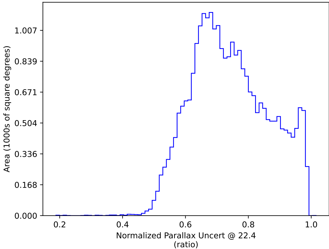
noroll_mjdp60_v3.4_10yrs All sky: Normalized Parallax Uncert @ 22.4
