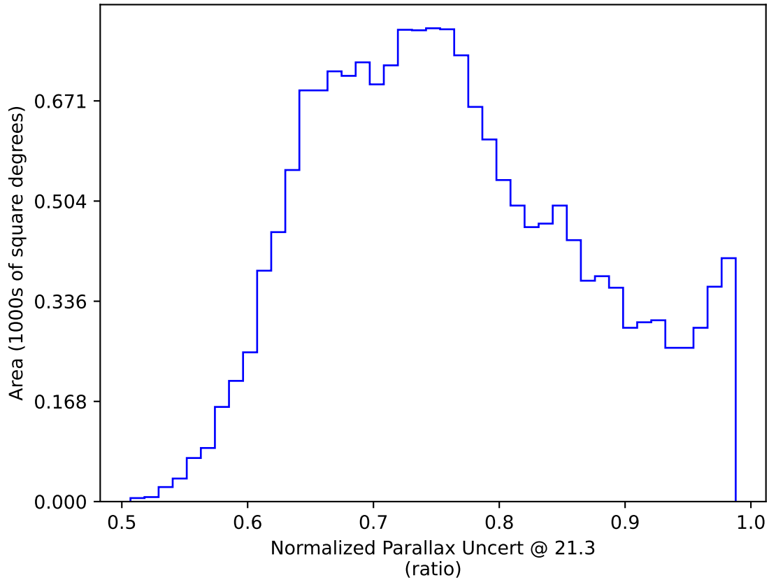
noroll_mjdp60_v3.4_10yrs WFD y band only: Normalized Parallax Uncert @ 21.3
