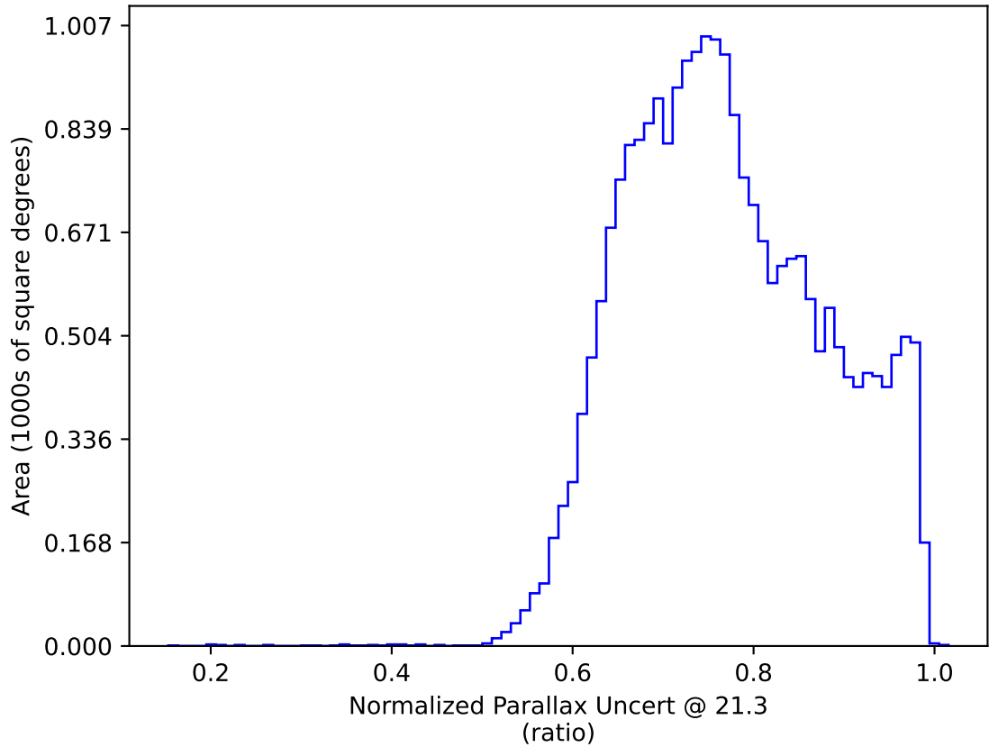
noroll_mjdp60_v3.4_10yrs All sky y band only: Normalized Parallax Uncert @ 21.3
