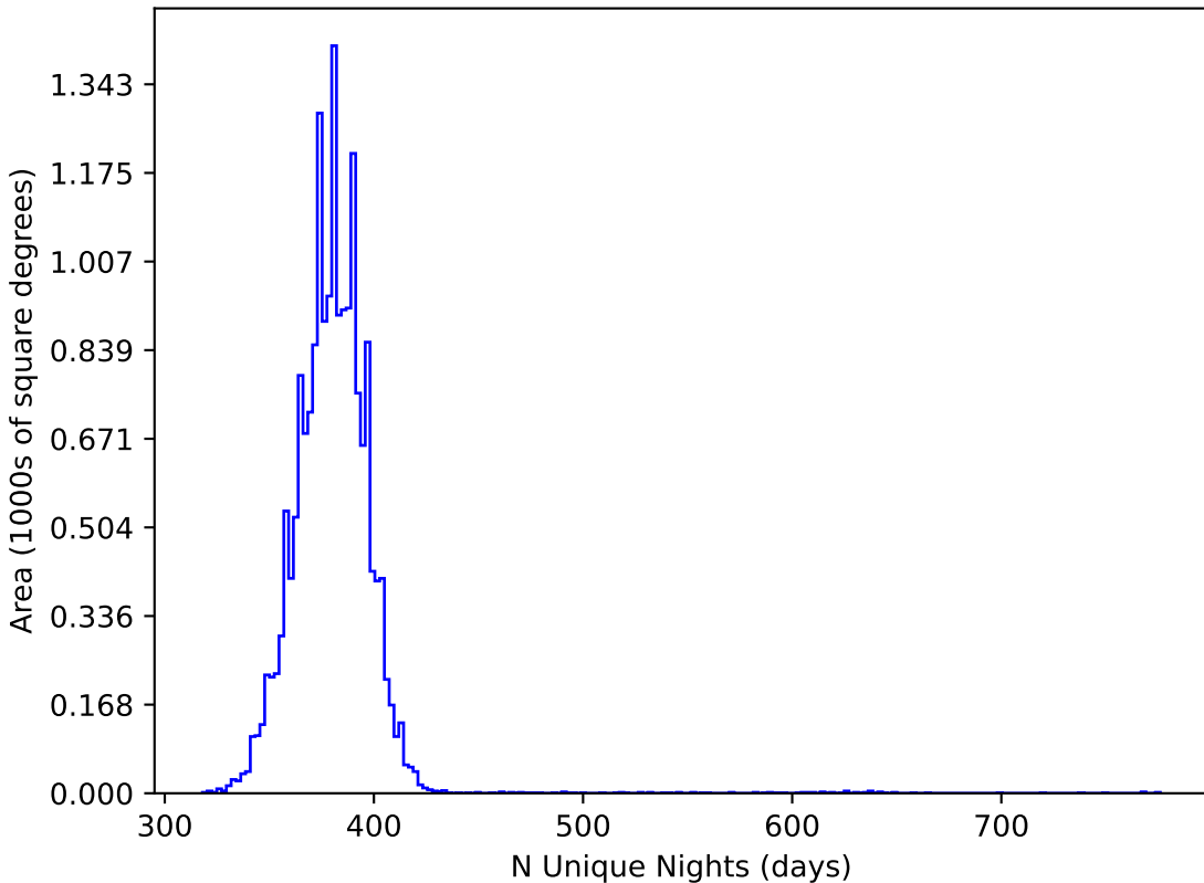
noroll_mjdp60_v3.4_10yrs WFD all bands: N Unique Nights
