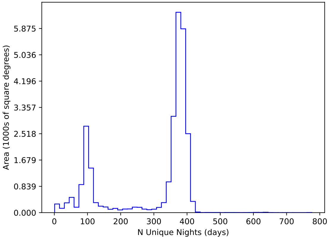
noroll_mjdp60_v3.4_10yrs All sky all bands: N Unique Nights
