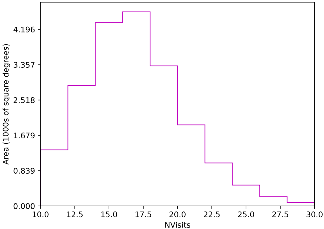
noroll_mjdp60_v3.4_10yrs Yr 3-4 z band: NVisits
