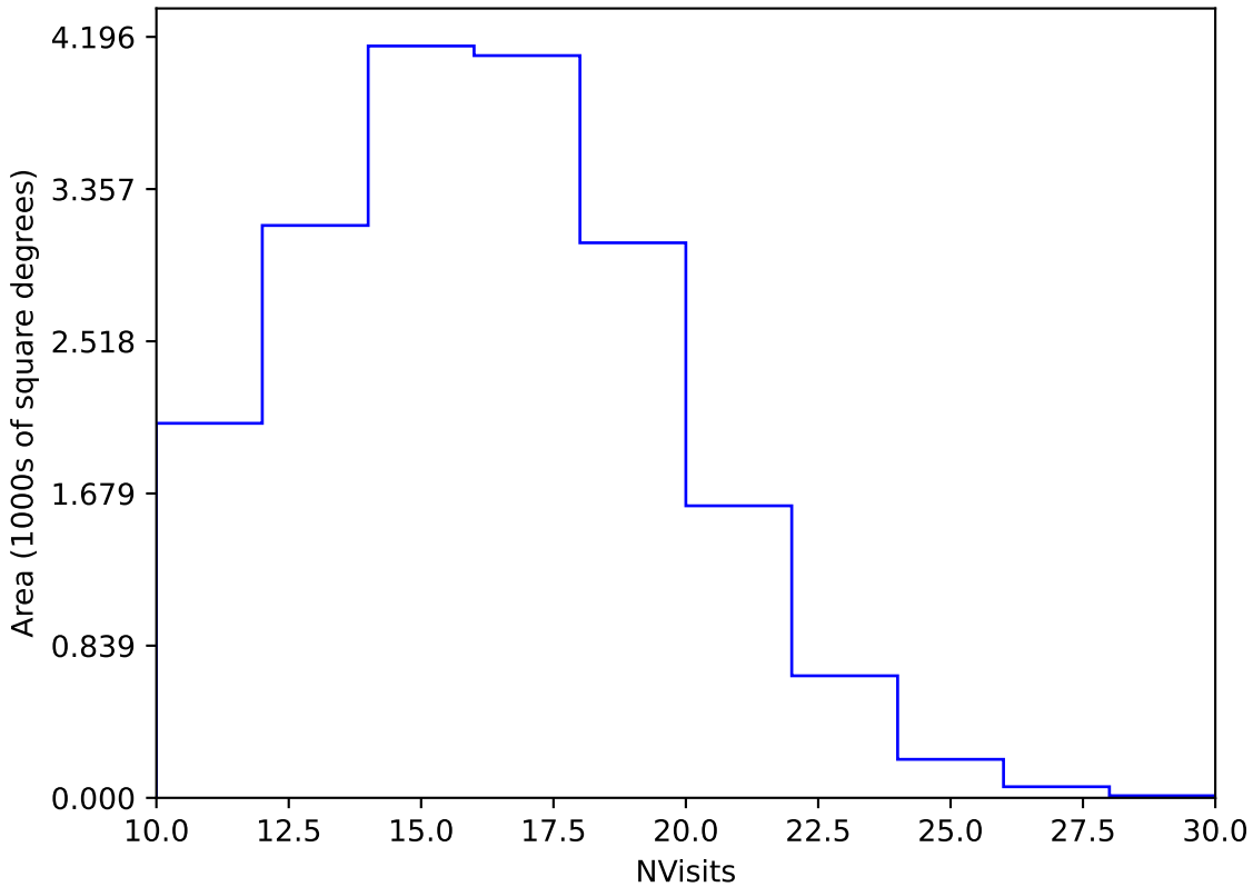
noroll_mjdp60_v3.4_10yrs Yr 3-4 y band: NVisits
