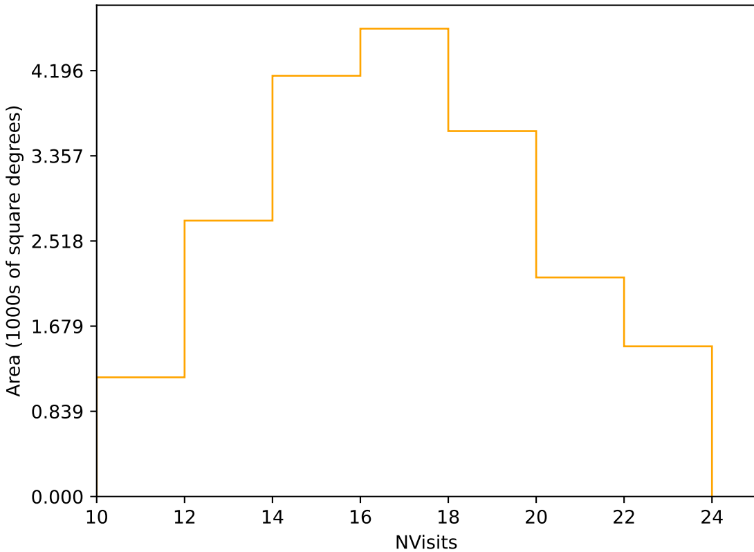
noroll_mjdp60_v3.4_10yrs Yr 3-4 r band: NVisits
