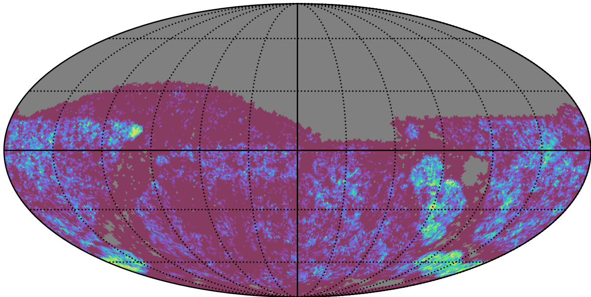
noroll_mjdp60_v3.4_10yrs Yr 3-4 g band: NVisits
