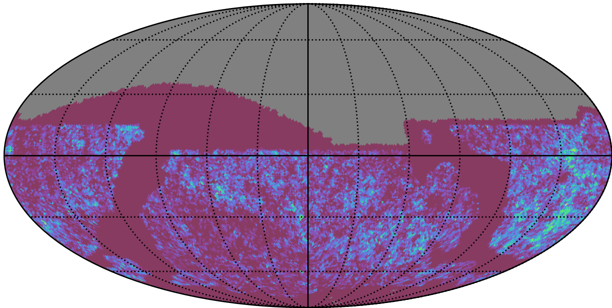
noroll_mjdp60_v3.4_10yrs Yr 3-4 all bands: NVisits
