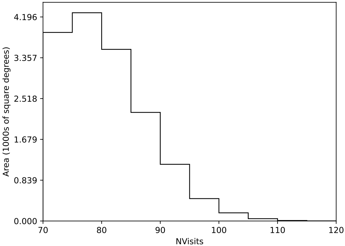
noroll_mjdp60_v3.4_10yrs Yr 3-4 all bands: NVisits
