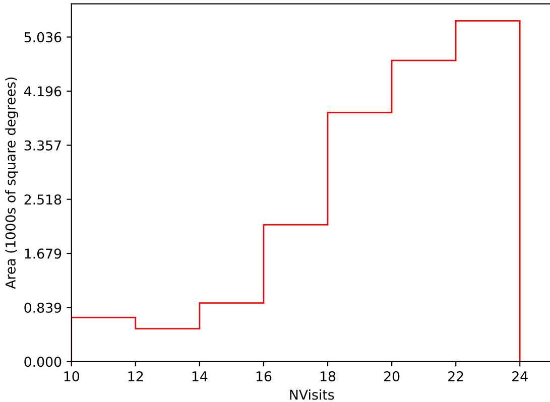
noroll_mjdp60_v3.4_10yrs Yr 1 i band: NVisits
