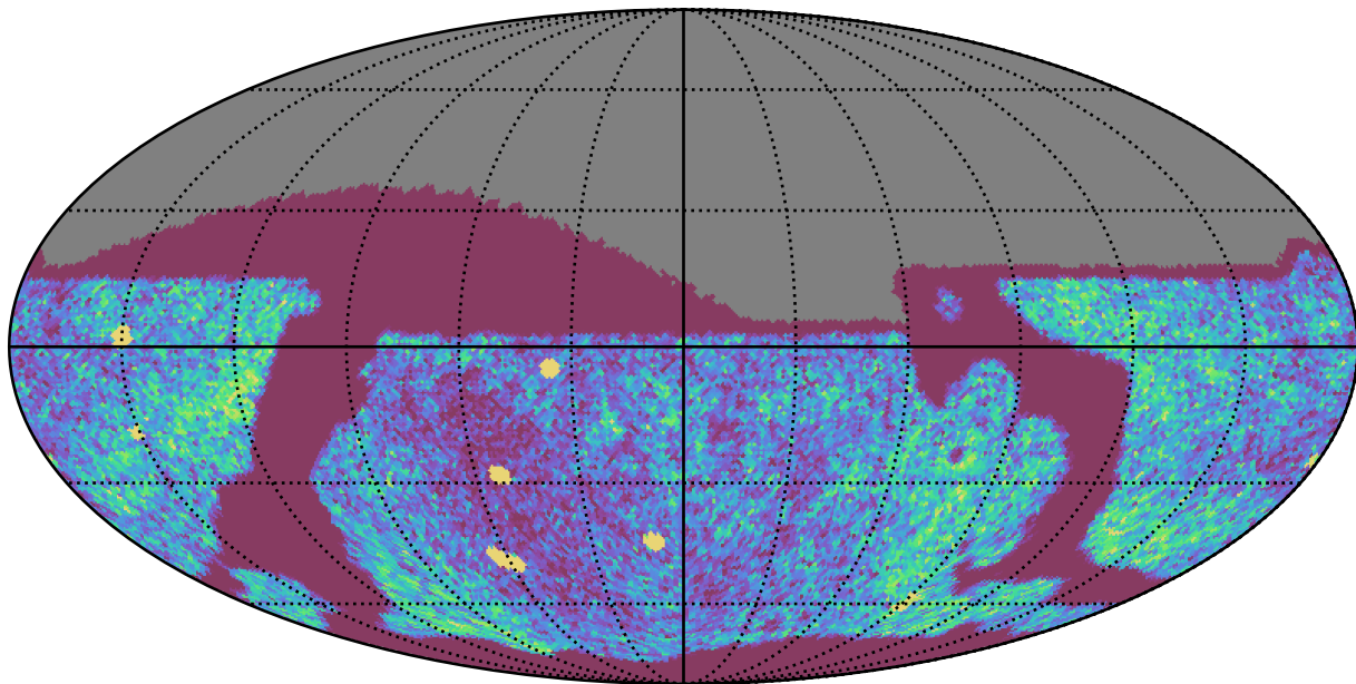
noroll_mjdp60_v3.4_10yrs Yr 1 all bands: NVisits
